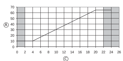
ECWS versus Input (mA)
