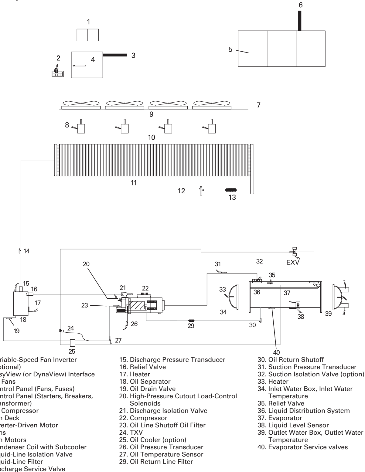
Figure 7 – System Schematic
