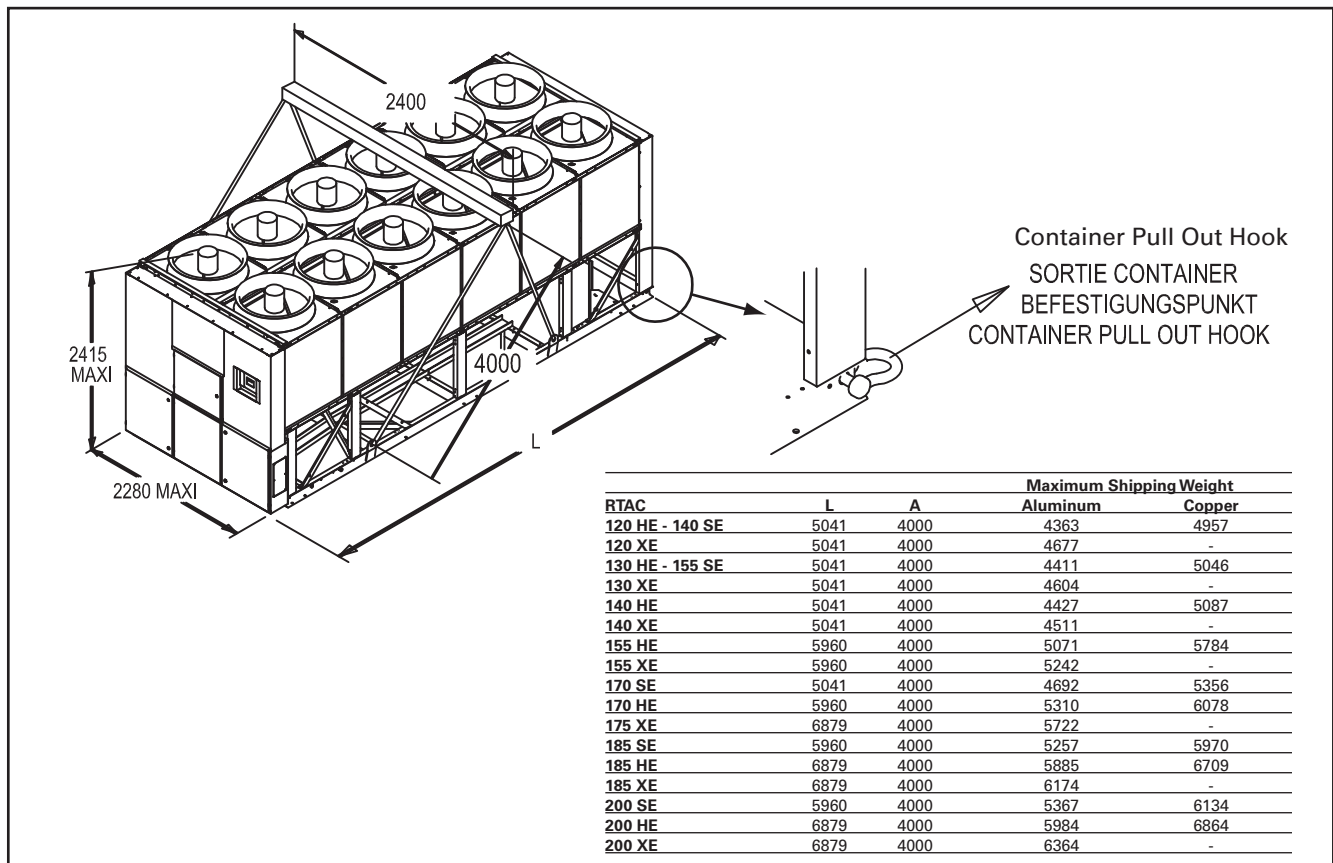
Figure 3 – Rigging the Unit, Sizes 120-200
