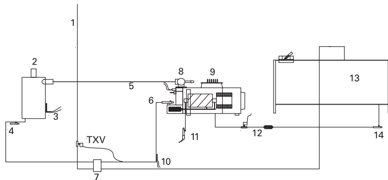
Figure 9 – Oil System Schematic
