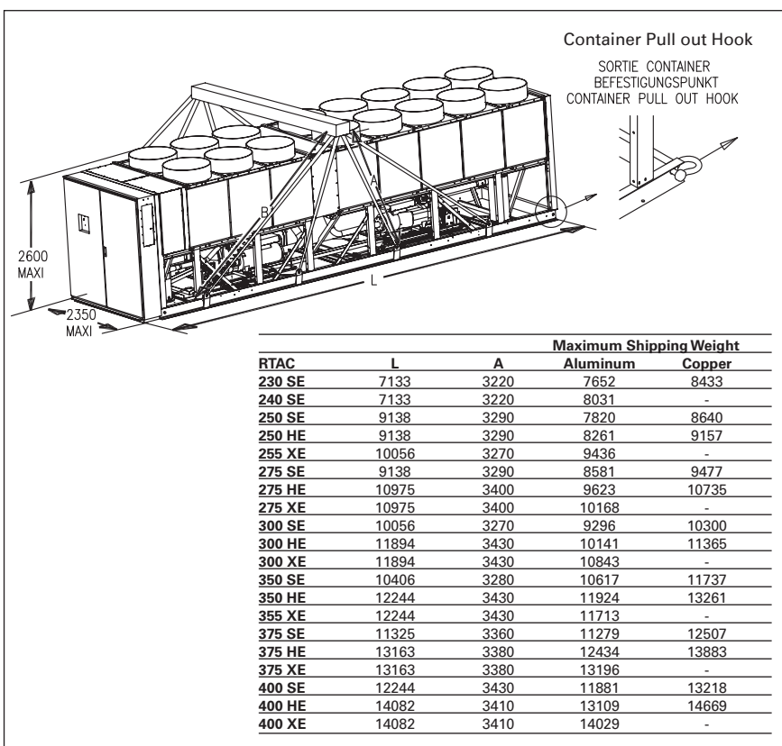
Figure 4 – Rigging the Unit, Sizes 230-400
