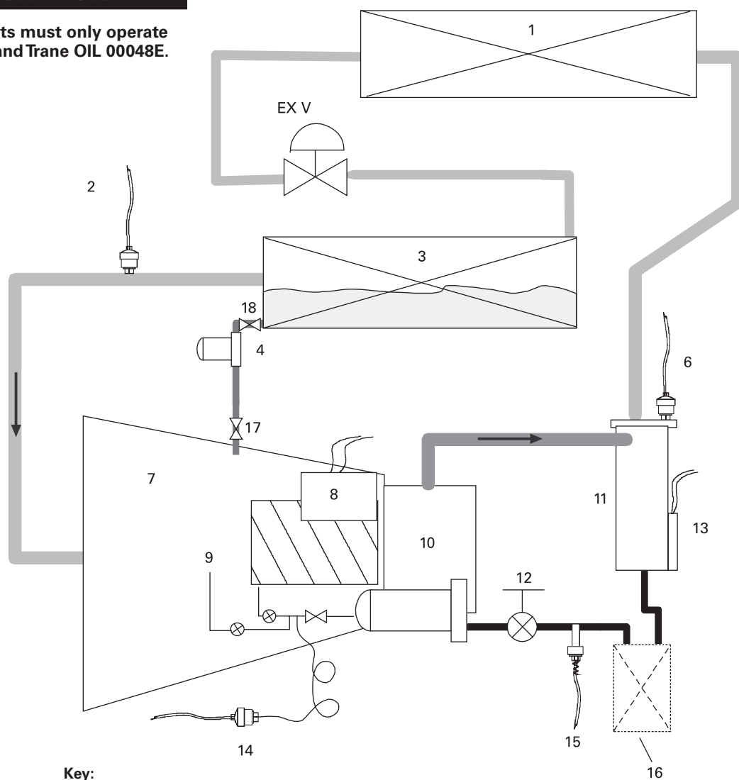
Figure 8 – RTAC Oil System
