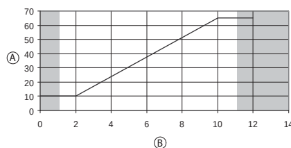
ECWS vs Input (VDC)
